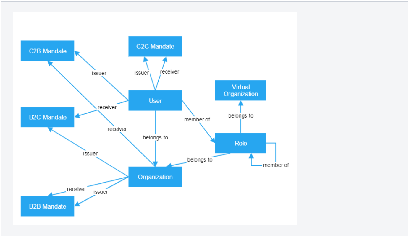
Figure 6. Simplified Conceptual Model with Member Of and Mandates
