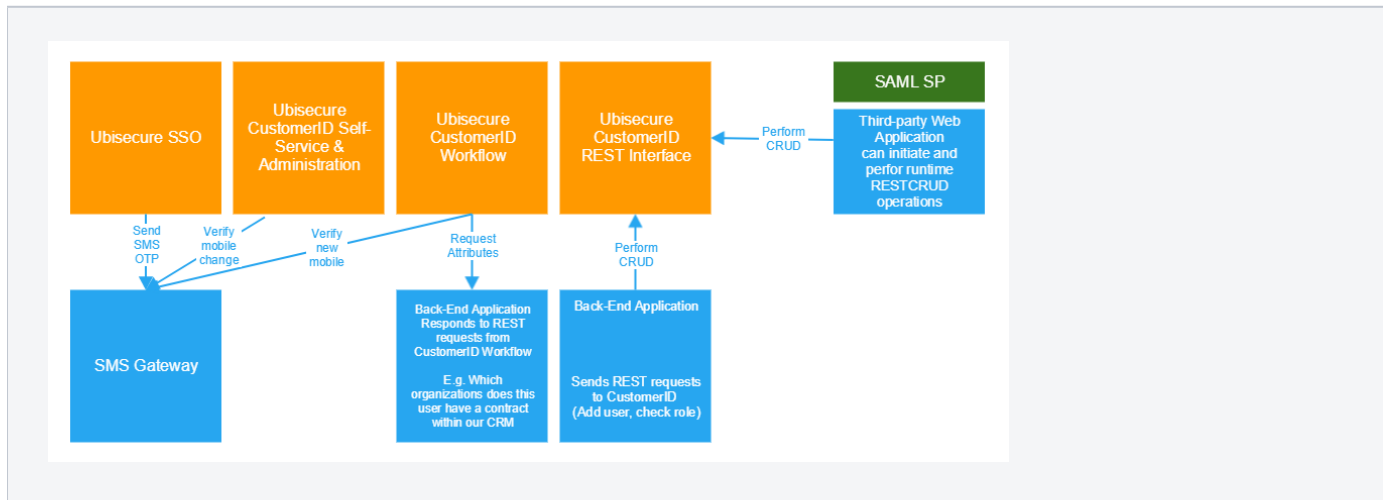
Figure 1. CustomerID Interfaces
